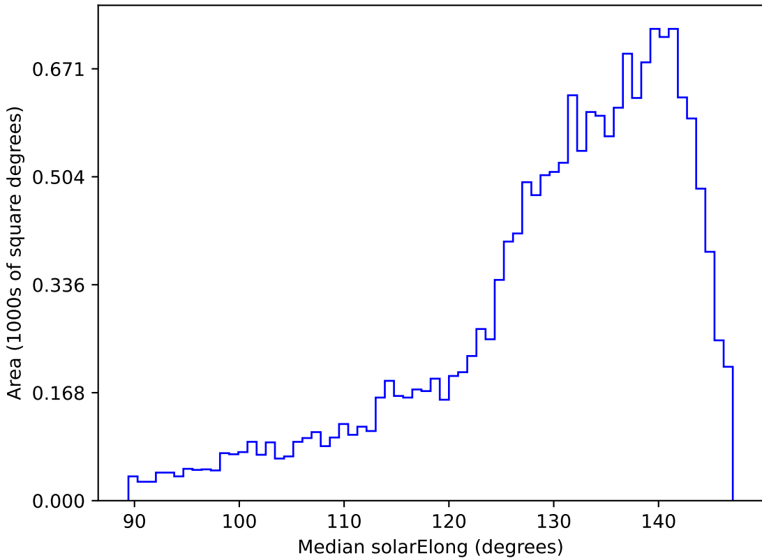
too_elab_r16_d3_gz_v3.4_10yrs WFD y band: Median solarElong
