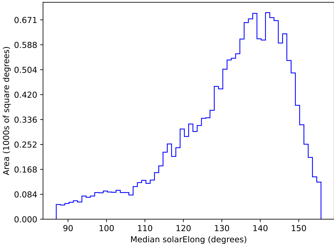
too_elab_r16_d3_gz_v3.4_10yrs WFD u band: Median solarElong
