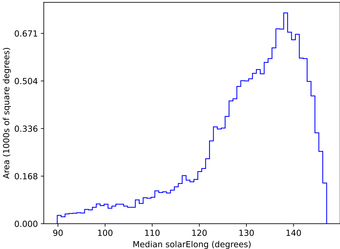
too_elab_r16_d3_gz_v3.4_10yrs WFD r band: Median solarElong
