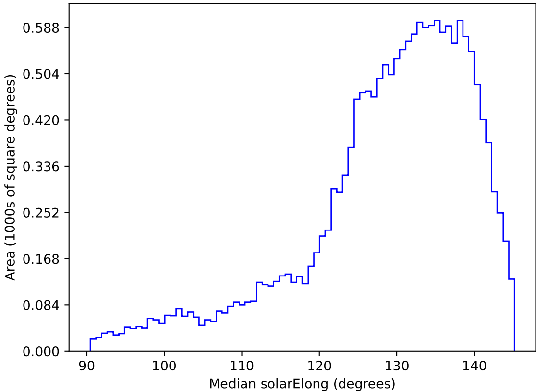
too_elab_r16_d3_gz_v3.4_10yrs WFD i band: Median solarElong
