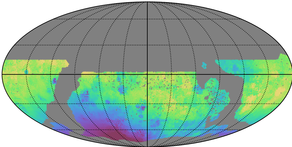
too_elab_r16_d3_gz_v3.4_10yrs WFD g band: Median solarElong
