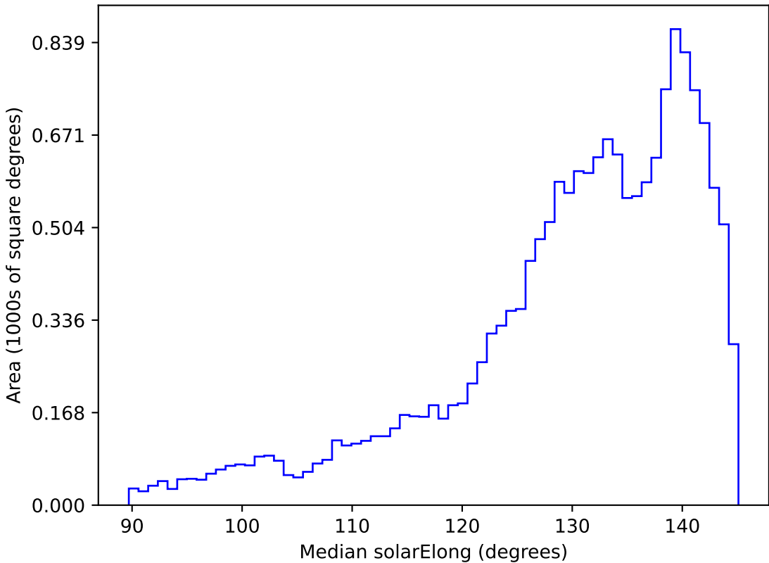
too_elab_r16_d3_gz_v3.4_10yrs WFD all bands: Median solarElong
