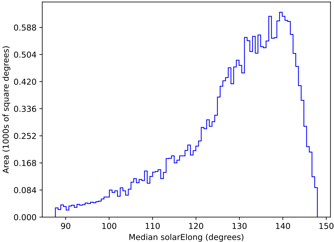
too_elab_r16_d3_gz_v3.4_10yrs All sky y band: Median solarElong
