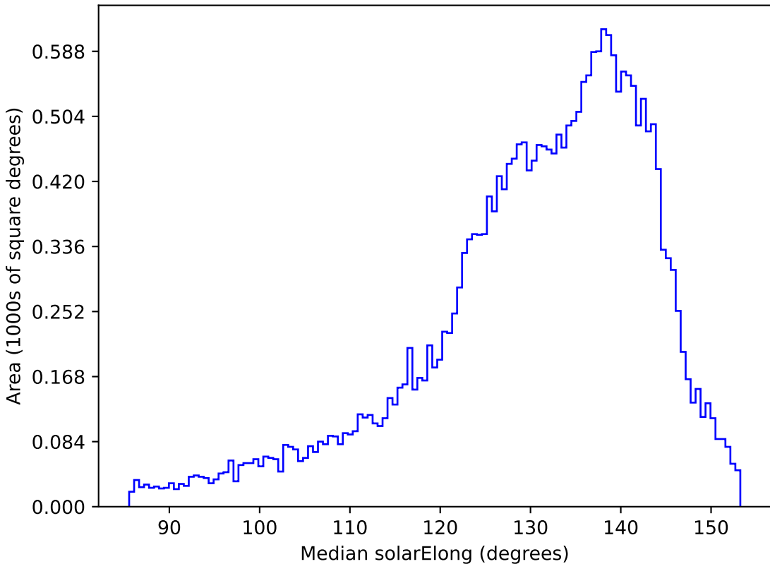
too_elab_r16_d3_gz_v3.4_10yrs All sky r band: Median solarElong
