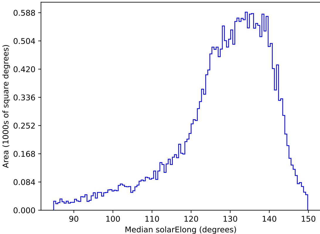
too_elab_r16_d3_gz_v3.4_10yrs All sky i band: Median solarElong
