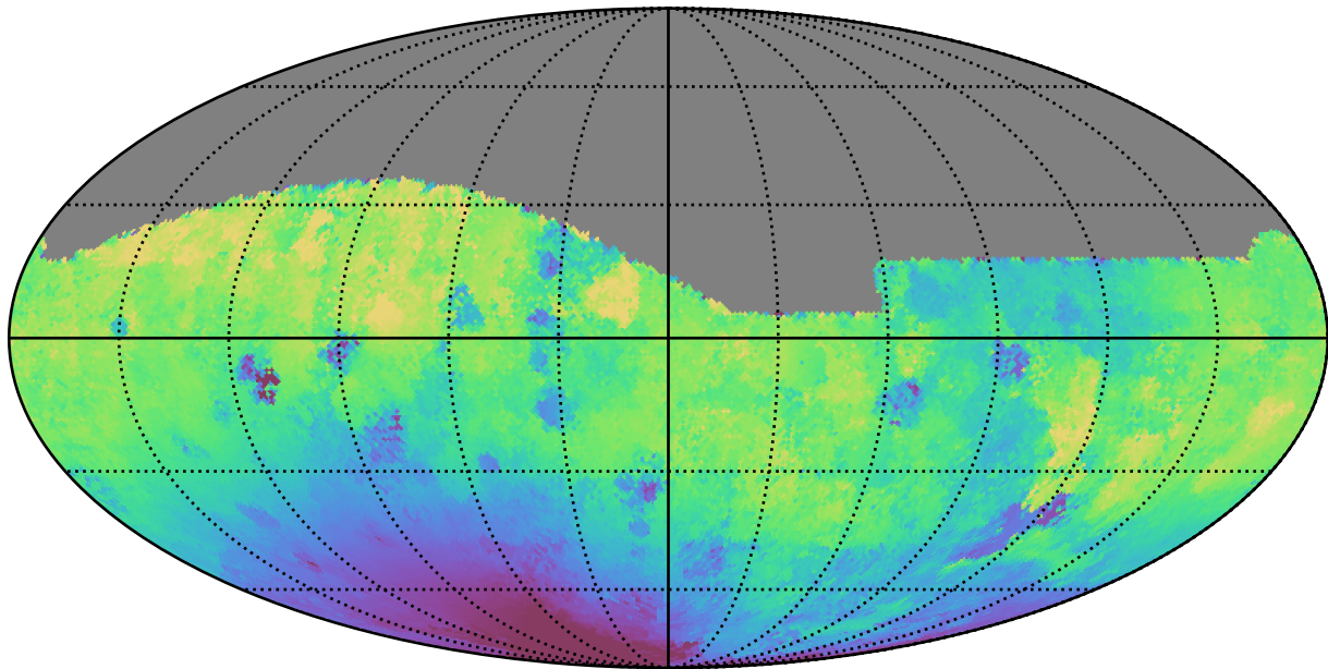
too_elab_r16_d3_gz_v3.4_10yrs All sky g band: Median solarElong
