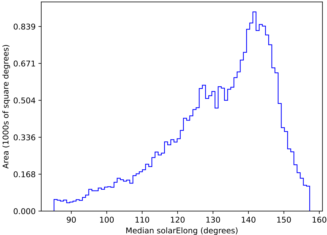
too_elab_r16_d3_gz_v3.4_10yrs All sky g band: Median solarElong
