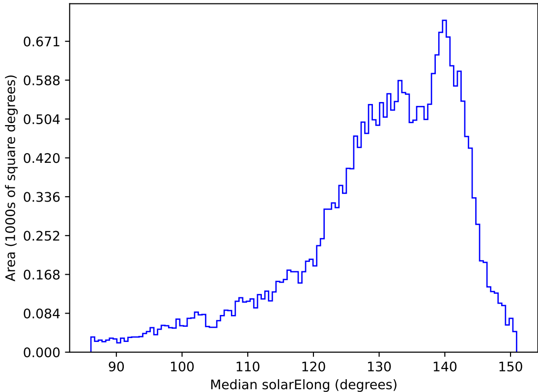
too_elab_r16_d3_gz_v3.4_10yrs All sky all bands: Median solarElong
