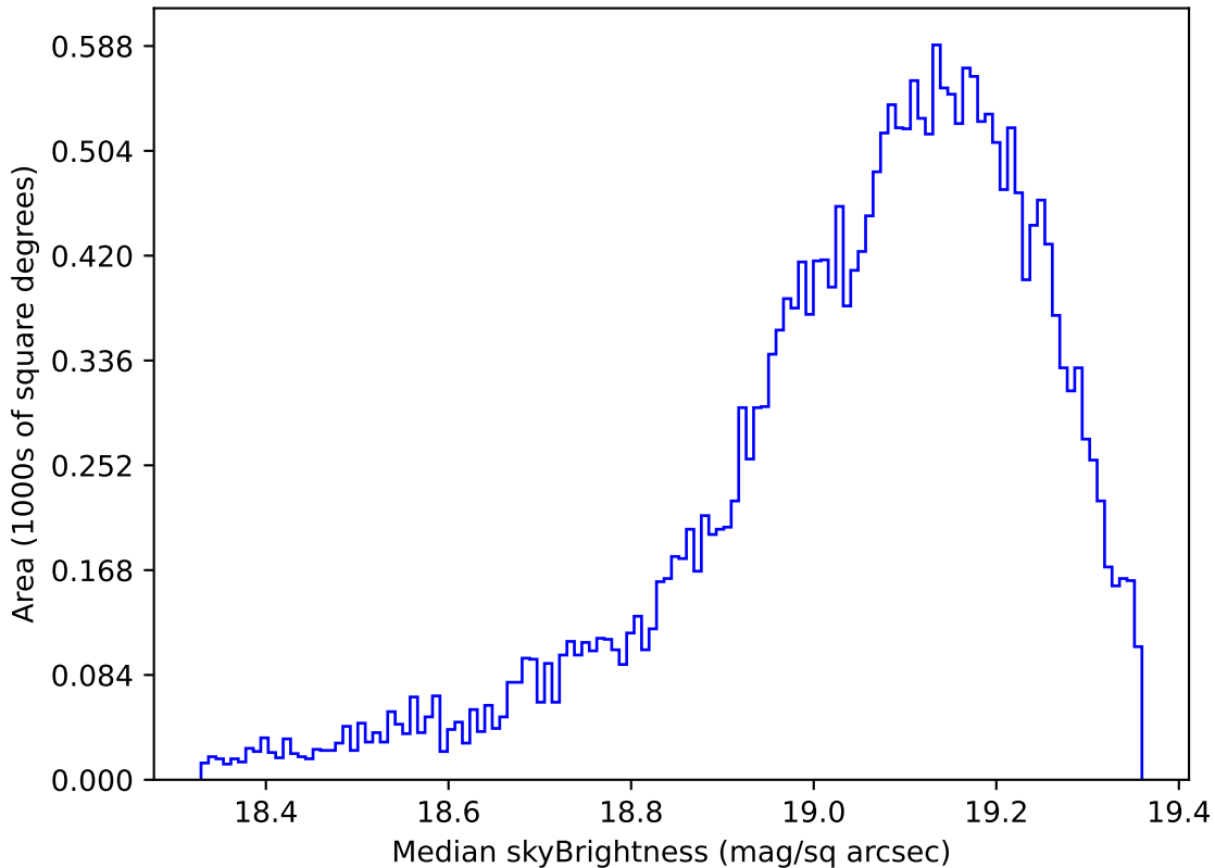
too_elab_r16_d3_gz_v3.4_10yrs Yr 1 z band: Median skyBrightness
