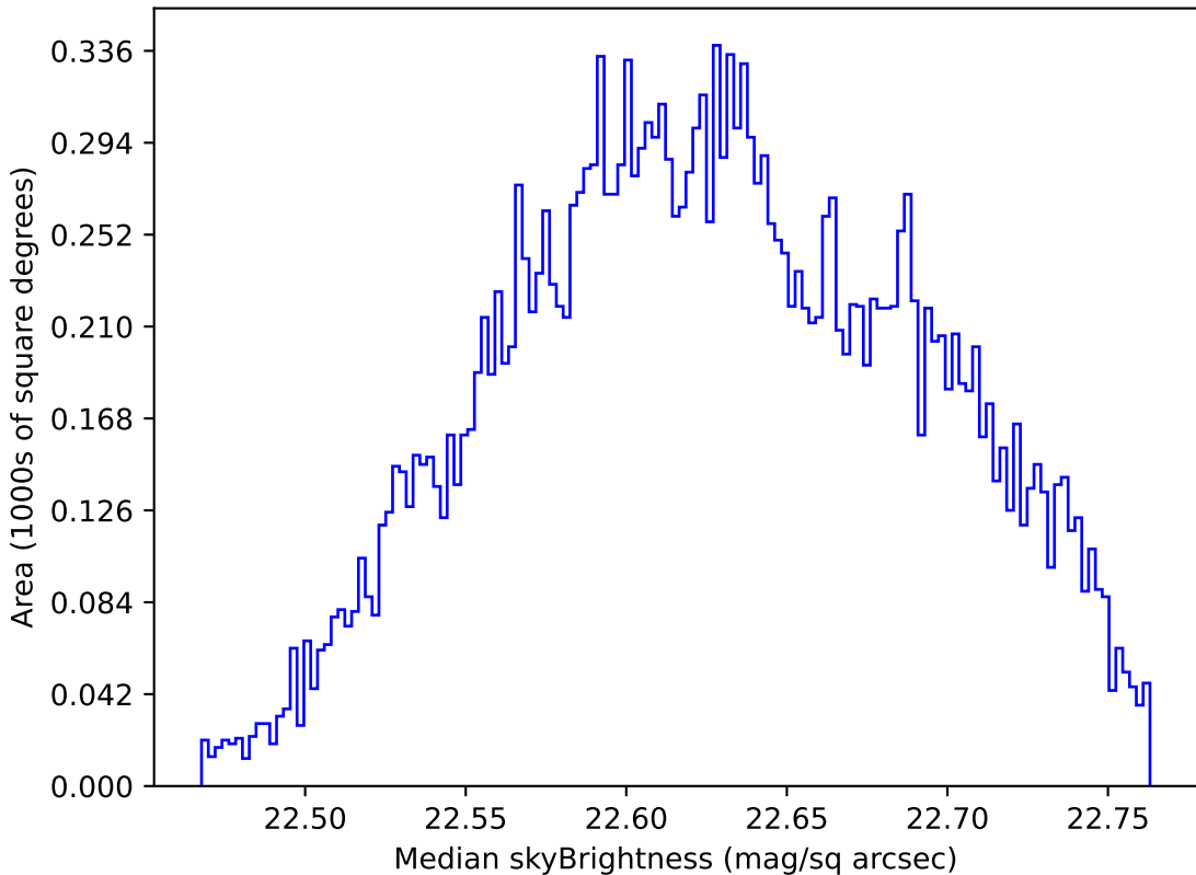
too_elab_r16_d3_gz_v3.4_10yrs Yr 1 u band: Median skyBrightness
