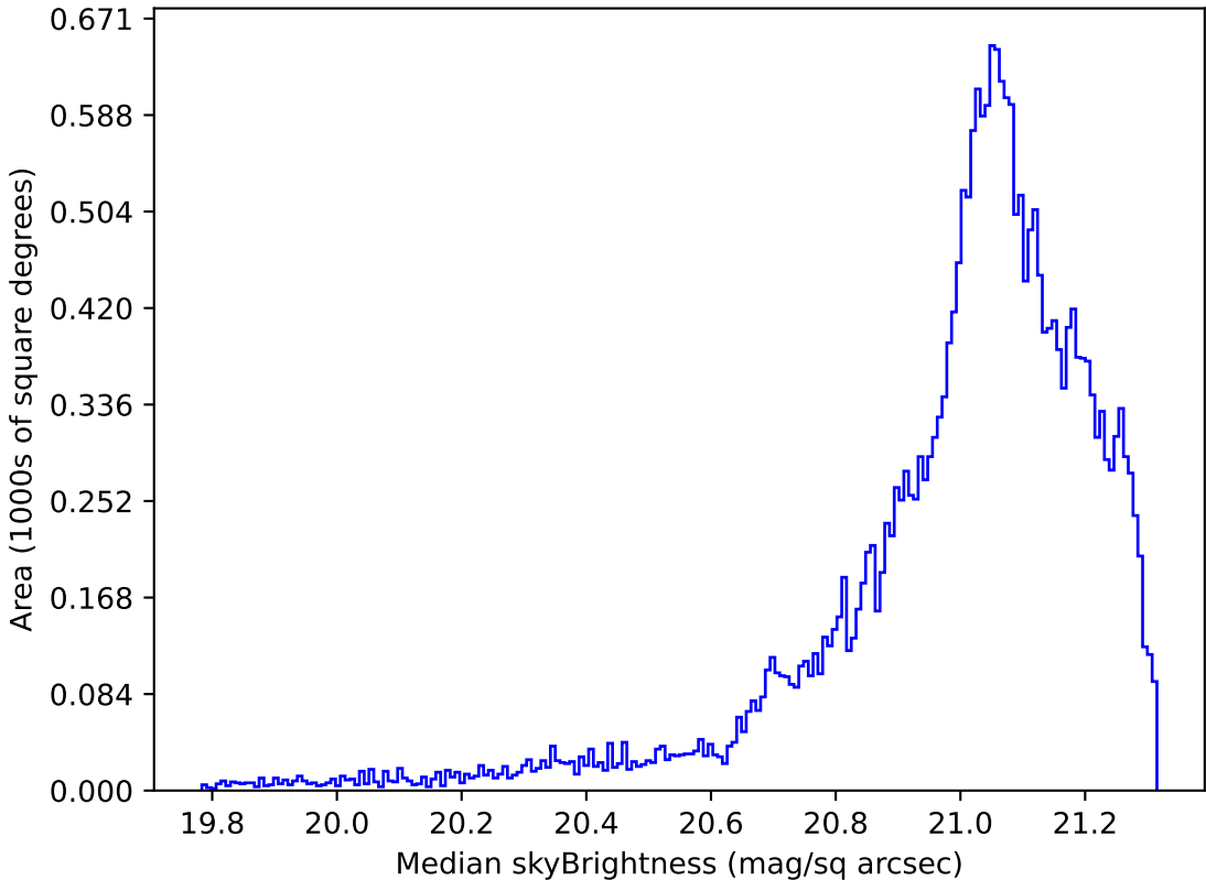
too_elab_r16_d3_gz_v3.4_10yrs Yr 1 r band: Median skyBrightness
