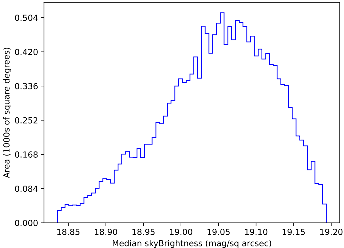
too_elab_r16_d3_gz_v3.4_10yrs WFD z band: Median skyBrightness
