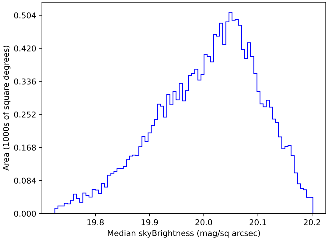
too_elab_r16_d3_gz_v3.4_10yrs WFD i band: Median skyBrightness
