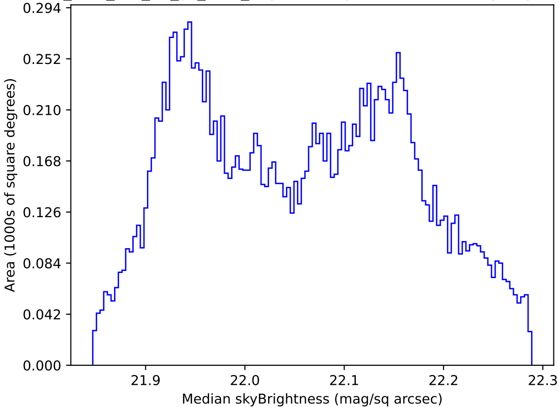
too_elab_r16_d3_gz_v3.4_10yrs WFD g band: Median skyBrightness
