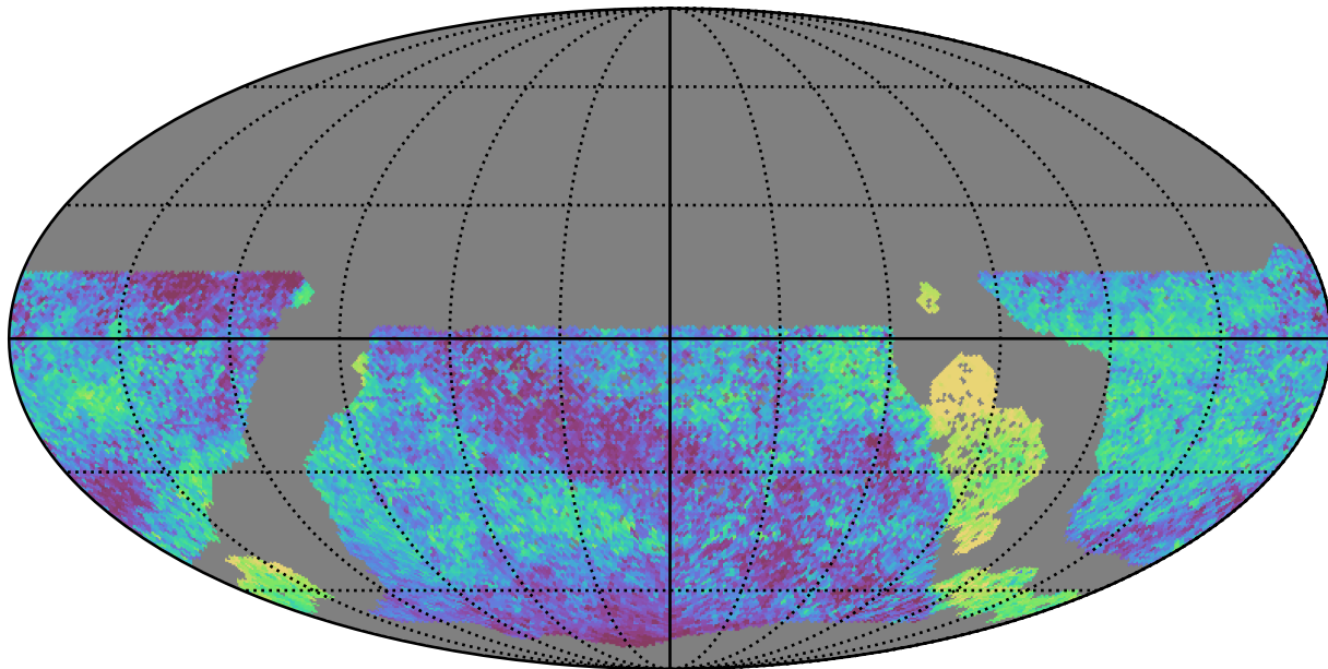
too_elab_r16_d3_gz_v3.4_10yrs WFD all bands: Median skyBrightness
