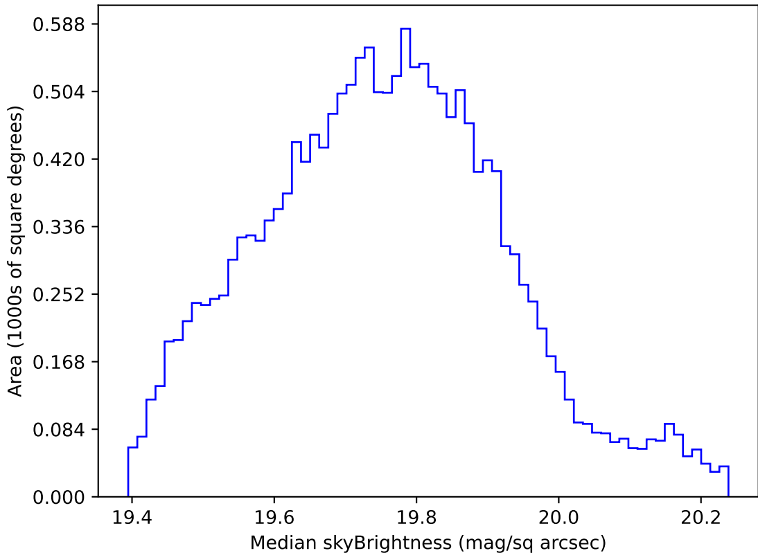
too_elab_r16_d3_gz_v3.4_10yrs WFD all bands: Median skyBrightness
