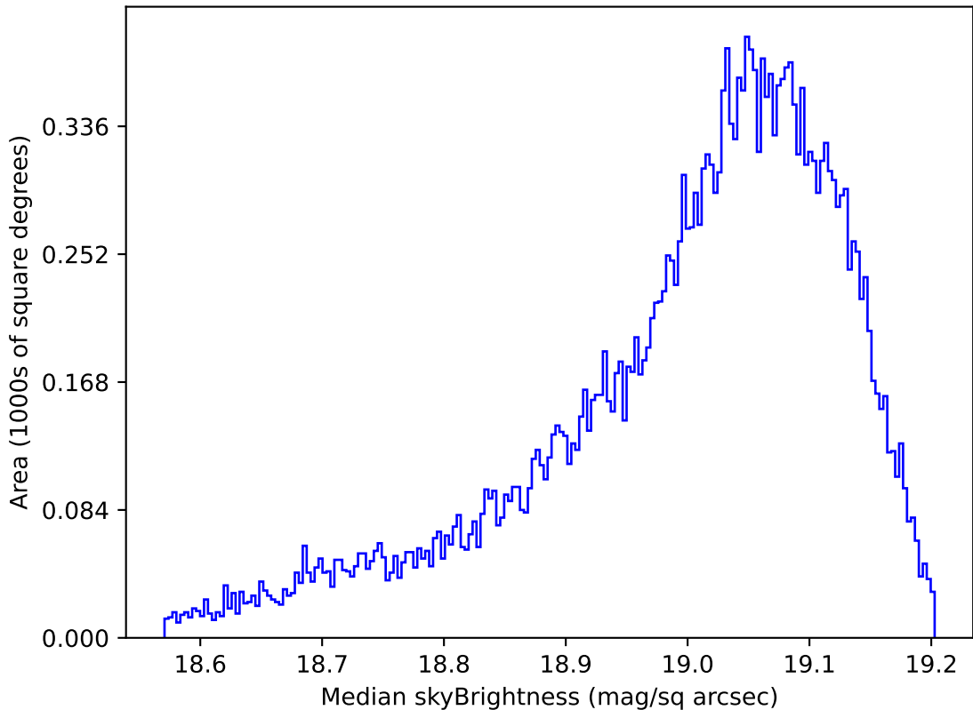
too_elab_r16_d3_gz_v3.4_10yrs All sky z band: Median skyBrightness
