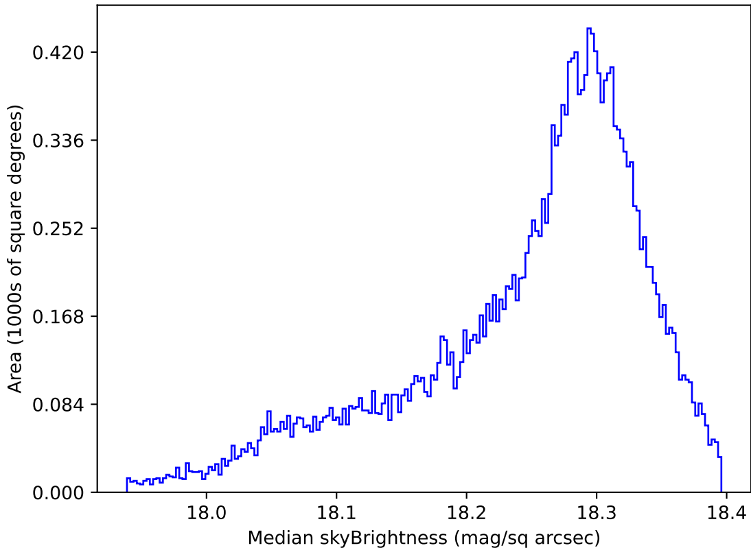
too_elab_r16_d3_gz_v3.4_10yrs All sky y band: Median skyBrightness
