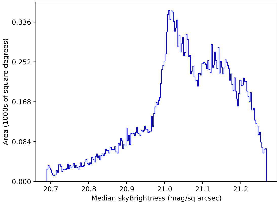
too_elab_r16_d3_gz_v3.4_10yrs All sky r band: Median skyBrightness
