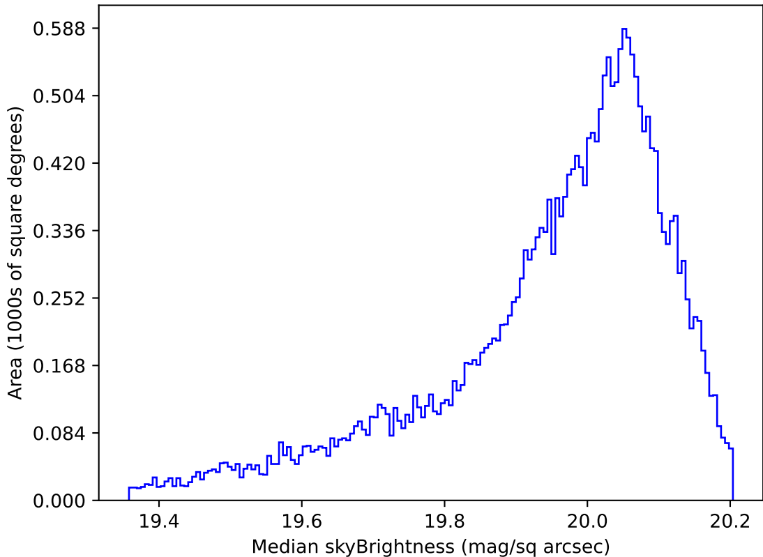
too_elab_r16_d3_gz_v3.4_10yrs All sky i band: Median skyBrightness
