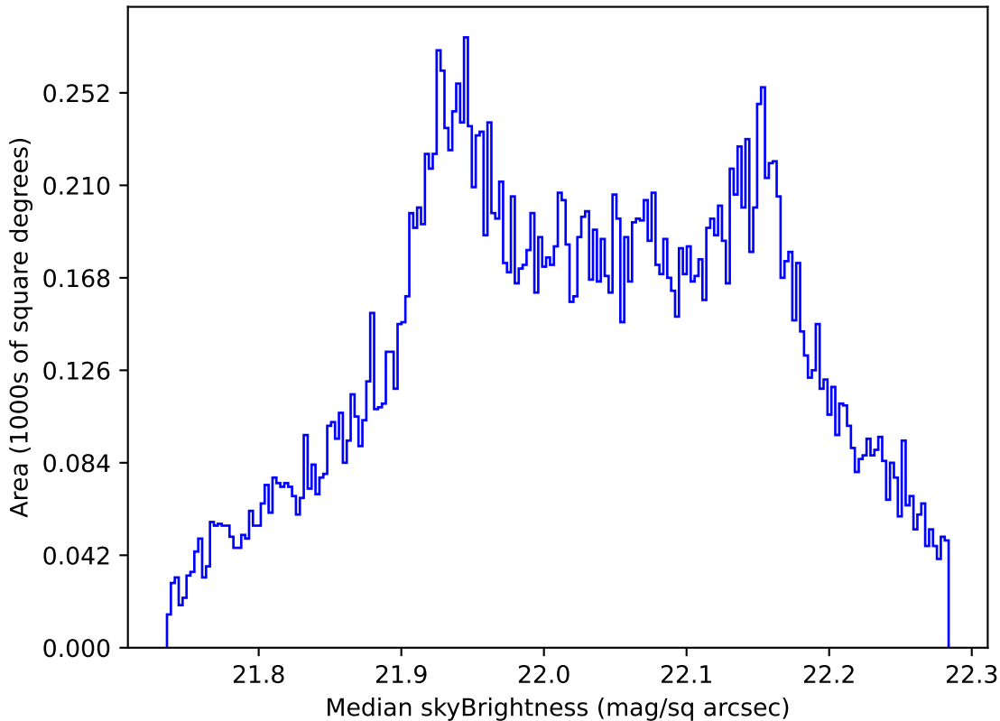
too_elab_r16_d3_gz_v3.4_10yrs All sky g band: Median skyBrightness
