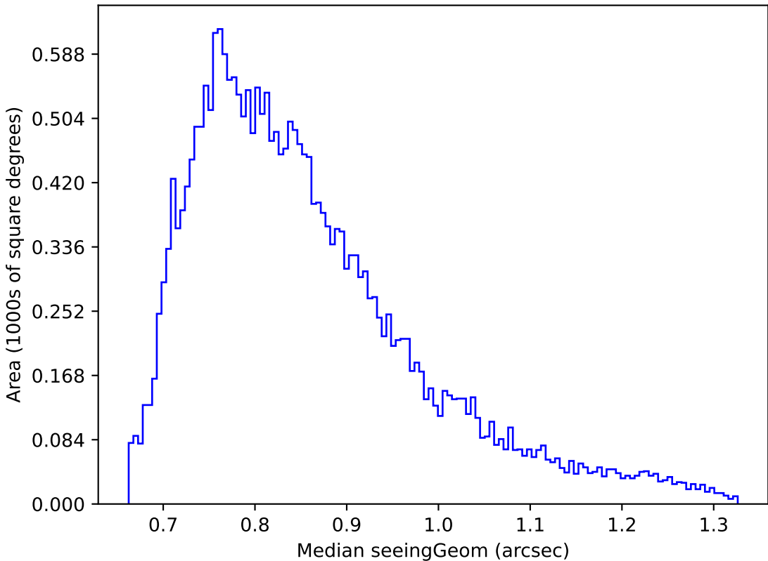
too_elab_r16_d3_gz_v3.4_10yrs Yr 1 r band: Median seeingGeom
