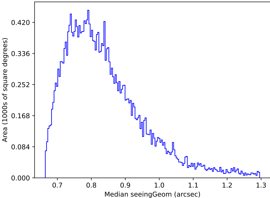
too_elab_r16_d3_gz_v3.4_10yrs Yr 1 i band: Median seeingGeom
