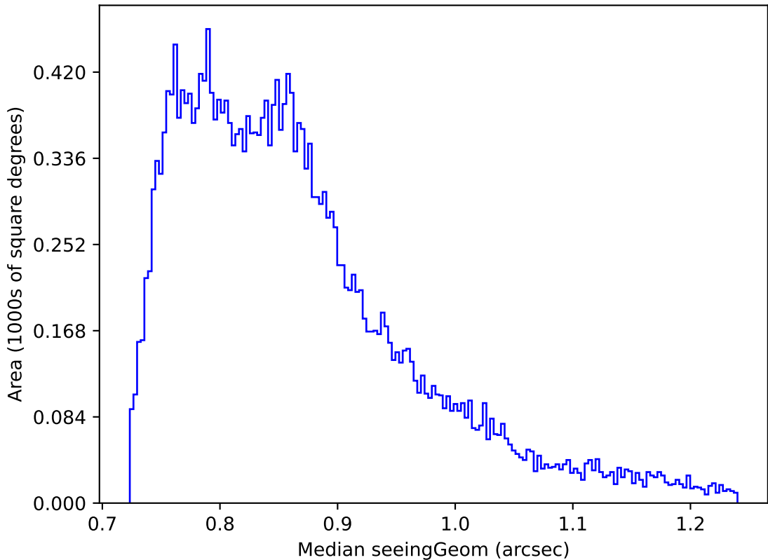
too_elab_r16_d3_gz_v3.4_10yrs Yr 1 all bands: Median seeingGeom
