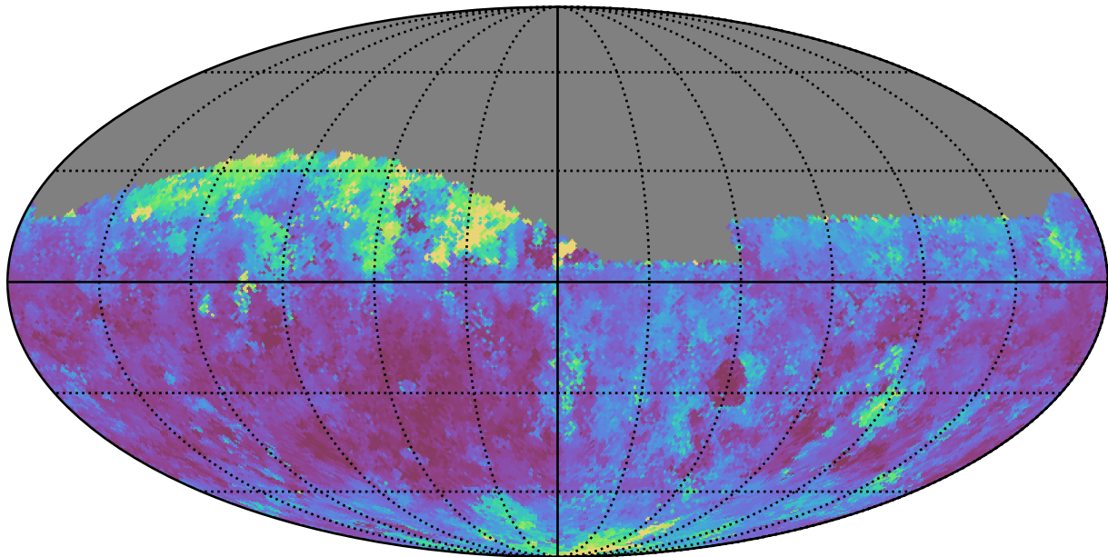
too_elab_r16_d3_gz_v3.4_10yrs Yr 1 z band: Median seeingEff
