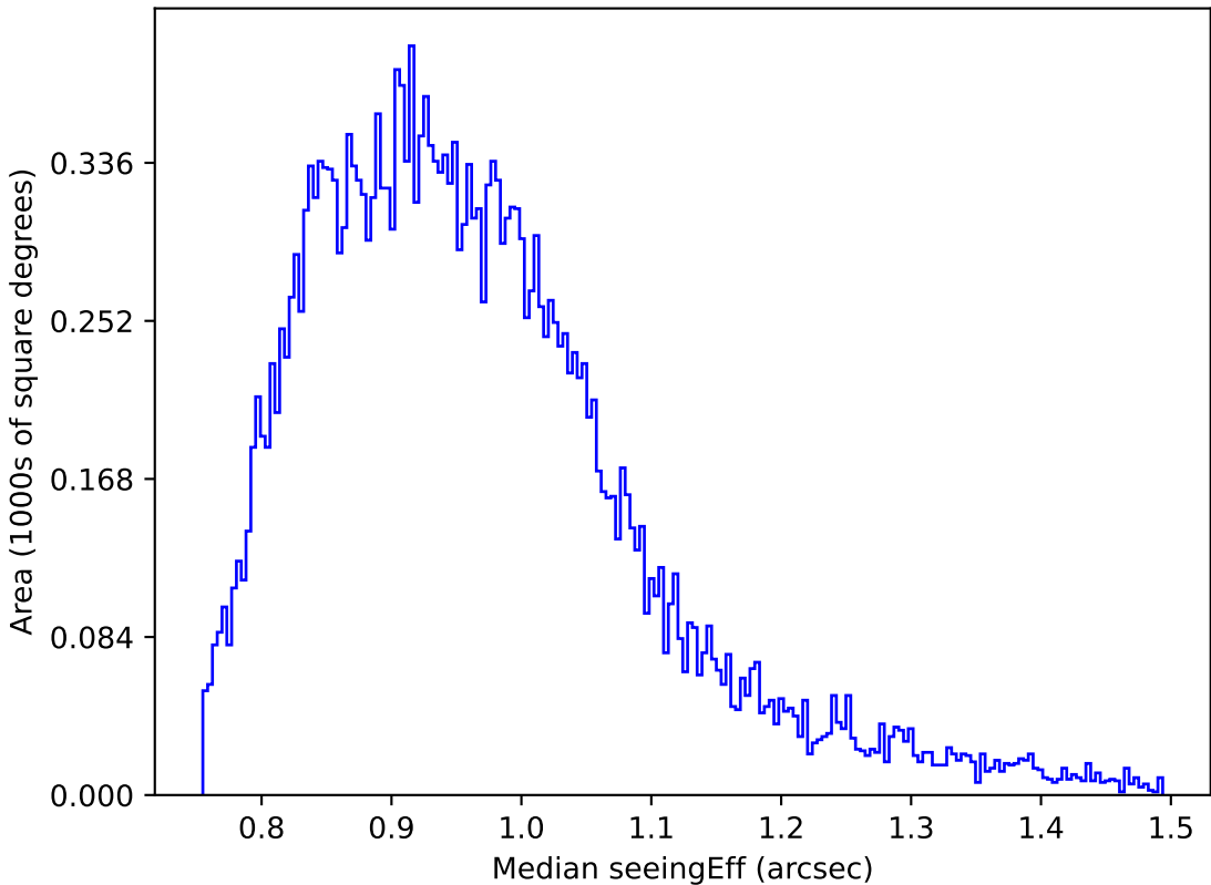
too_elab_r16_d3_gz_v3.4_10yrs Yr 1 z band: Median seeingEff
