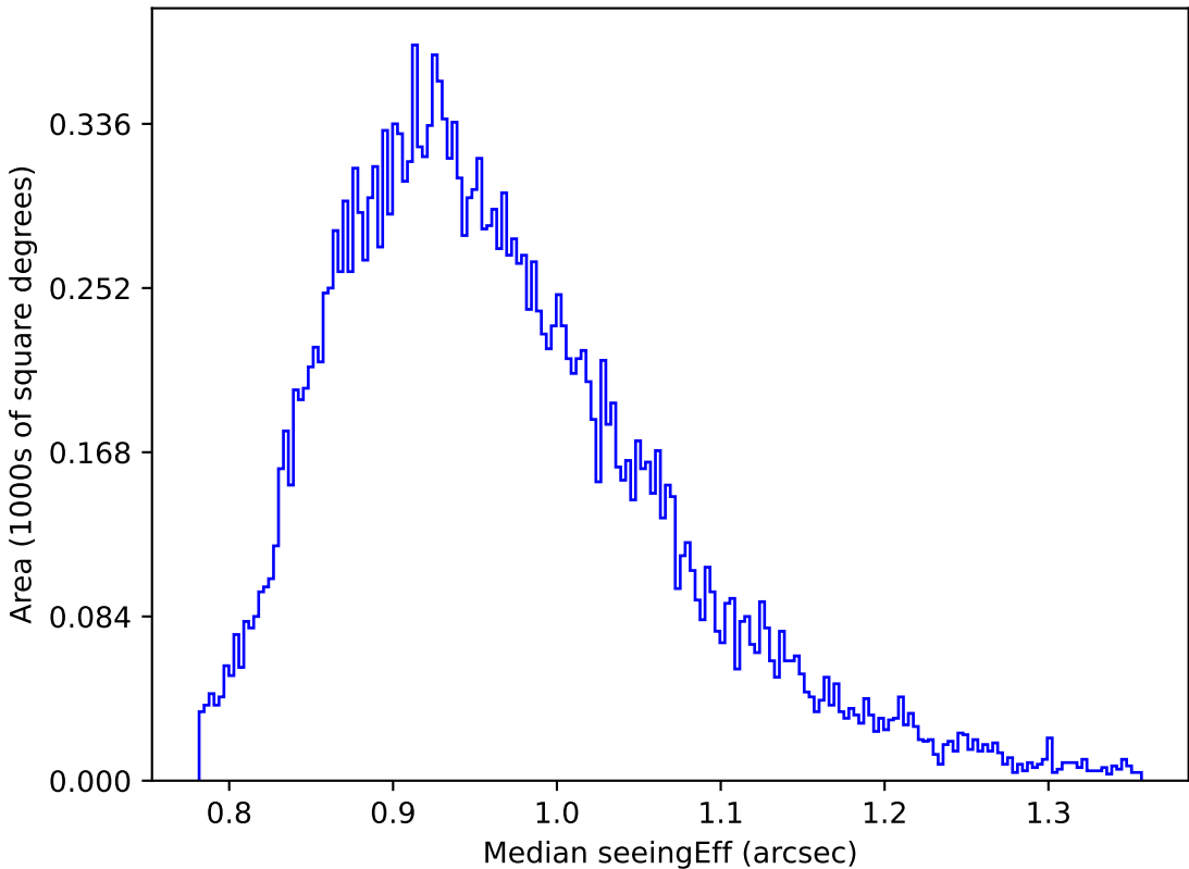
too_elab_r16_d3_gz_v3.4_10yrs Yr 1 y band: Median seeingEff
