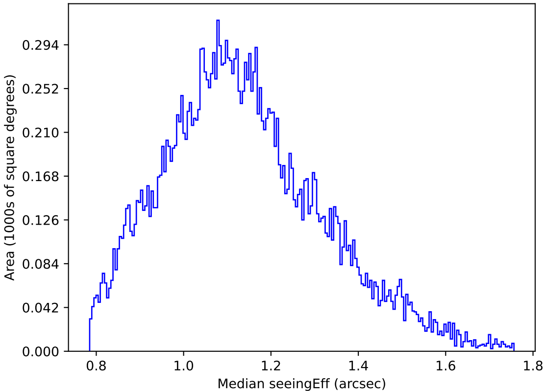
too_elab_r16_d3_gz_v3.4_10yrs Yr 1 u band: Median seeingEff
