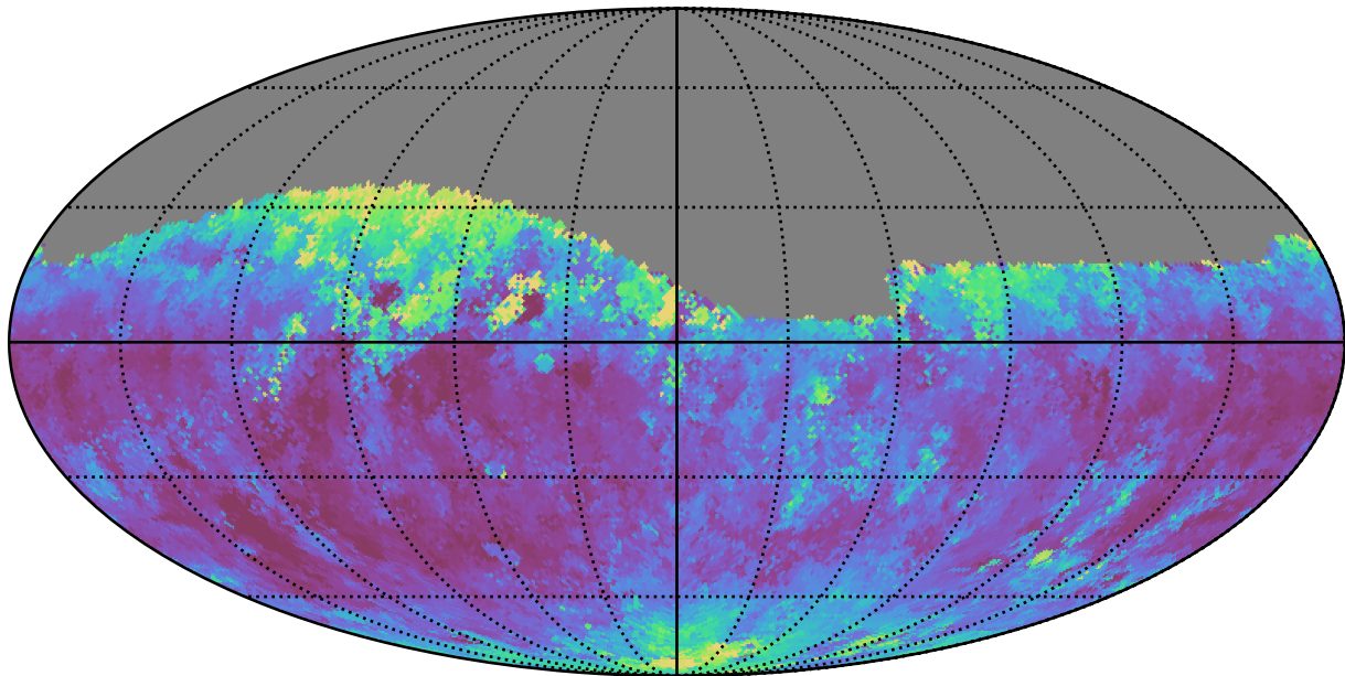
too_elab_r16_d3_gz_v3.4_10yrs Yr 1 r band: Median seeingEff
