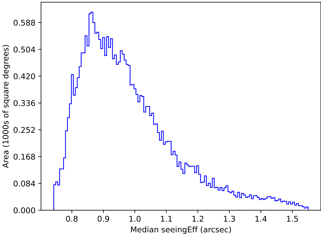
too_elab_r16_d3_gz_v3.4_10yrs Yr 1 r band: Median seeingEff
