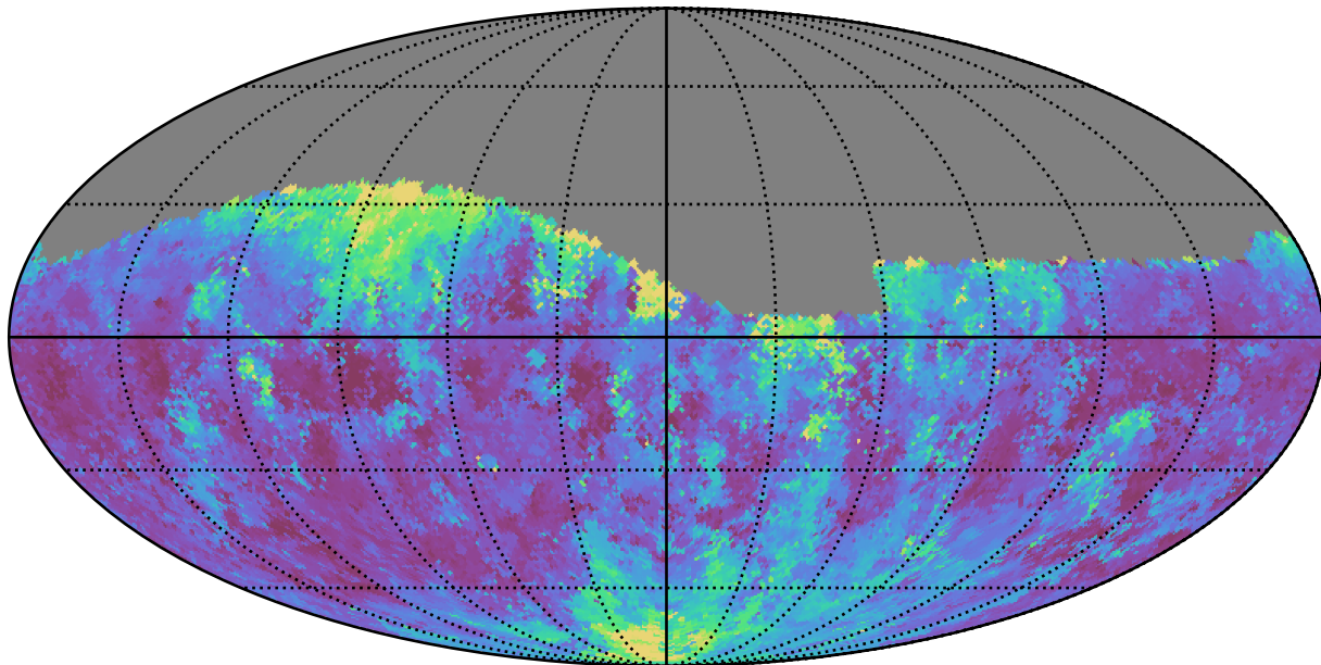
too_elab_r16_d3_gz_v3.4_10yrs Yr 1 g band: Median seeingEff
