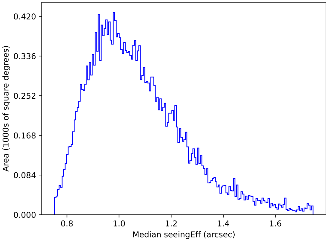
too_elab_r16_d3_gz_v3.4_10yrs Yr 1 g band: Median seeingEff
