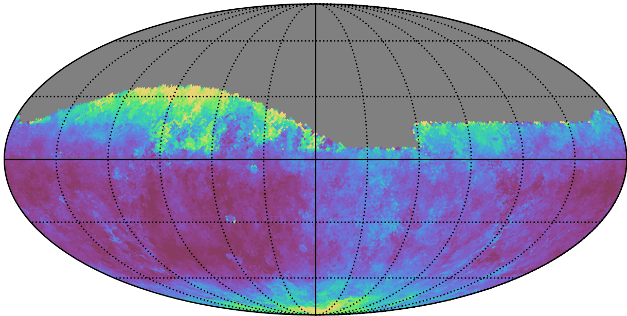
too_elab_r16_d3_gz_v3.4_10yrs Yr 1 all bands: Median seeingEff
