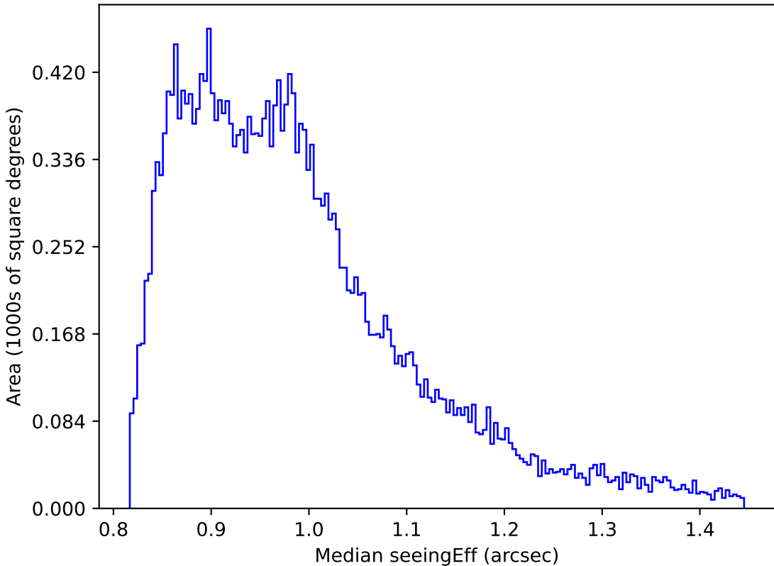
too_elab_r16_d3_gz_v3.4_10yrs Yr 1 all bands: Median seeingEff
