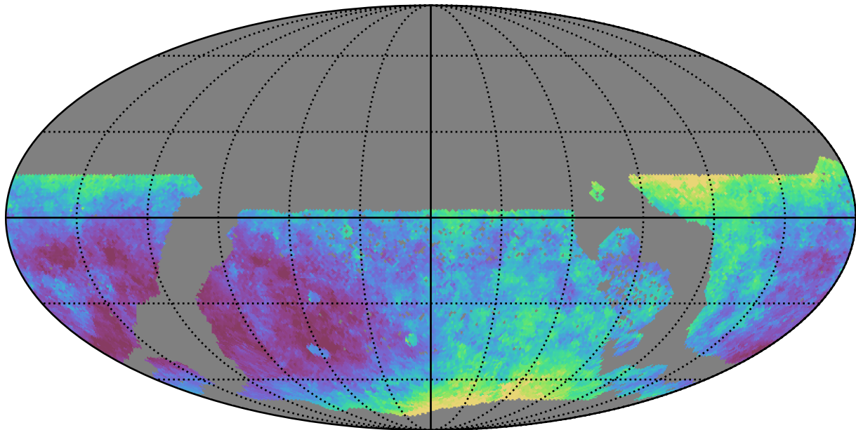
too_elab_r16_d3_gz_v3.4_10yrs WFD z band: Median seeingEff
