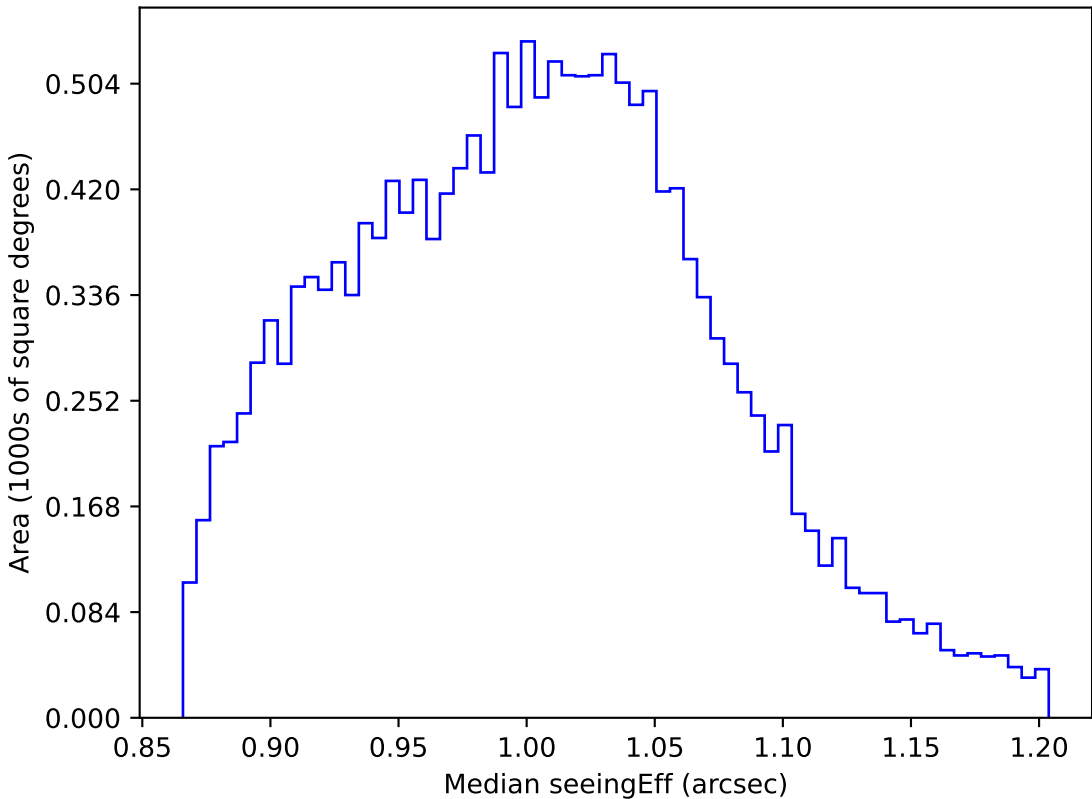
too_elab_r16_d3_gz_v3.4_10yrs WFD z band: Median seeingEff
