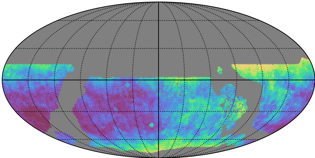
too_elab_r16_d3_gz_v3.4_10yrs WFD y band: Median seeingEff
