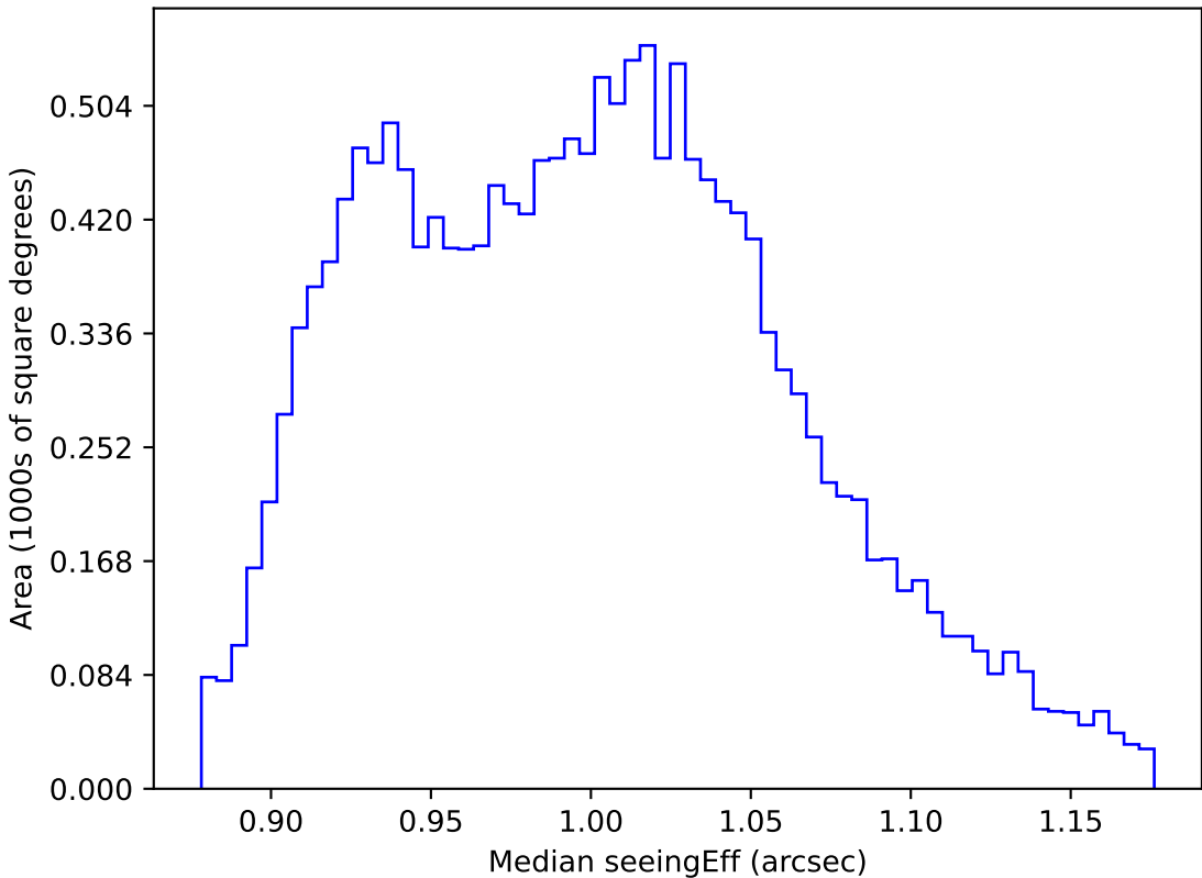
too_elab_r16_d3_gz_v3.4_10yrs WFD y band: Median seeingEff
