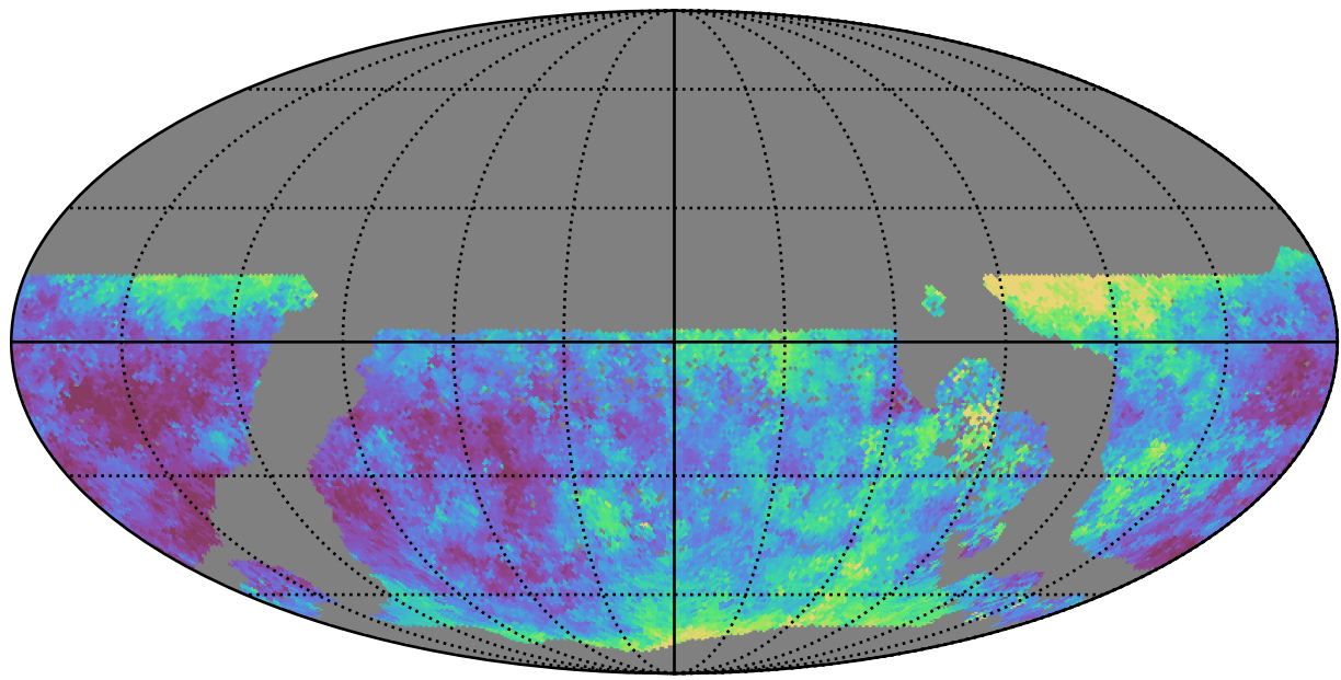
too_elab_r16_d3_gz_v3.4_10yrs WFD u band: Median seeingEff
