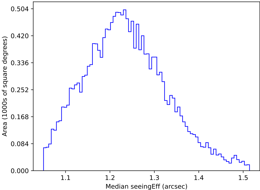
too_elab_r16_d3_gz_v3.4_10yrs WFD u band: Median seeingEff
