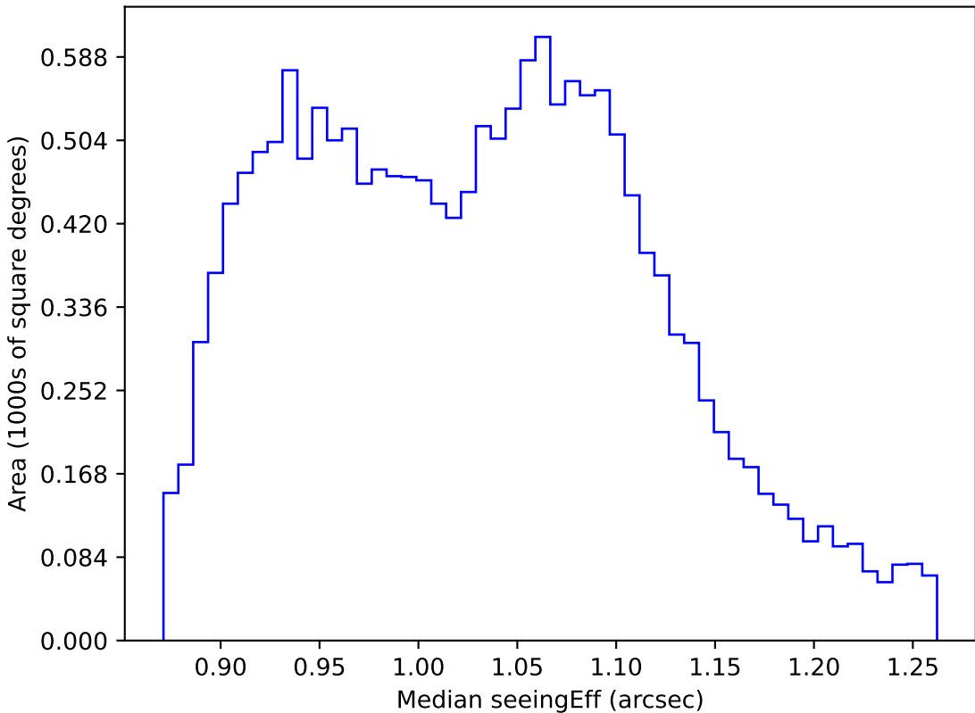
too_elab_r16_d3_gz_v3.4_10yrs WFD r band: Median seeingEff
