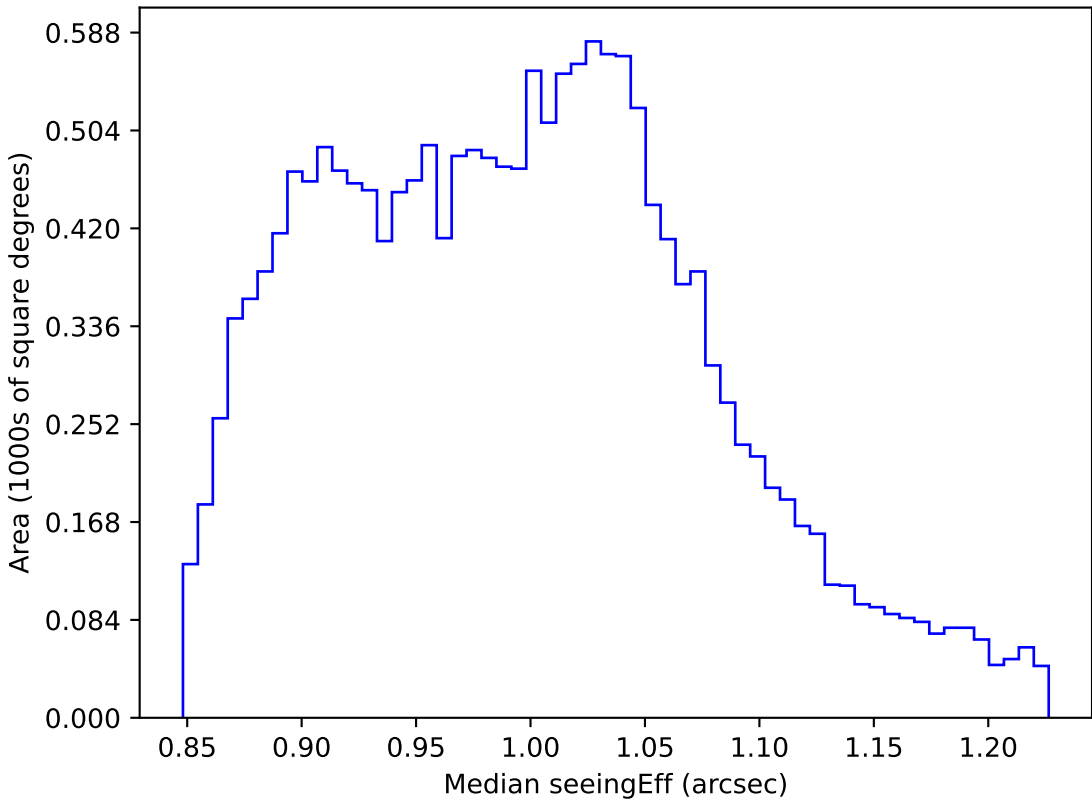
too_elab_r16_d3_gz_v3.4_10yrs WFD i band: Median seeingEff
