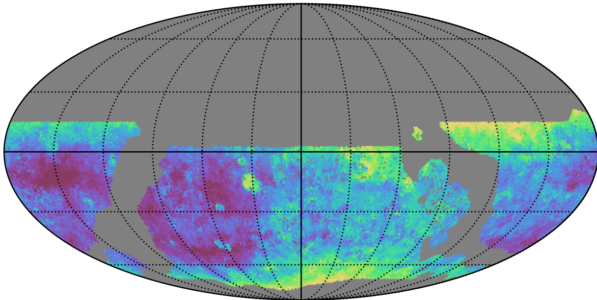
too_elab_r16_d3_gz_v3.4_10yrs WFD g band: Median seeingEff
