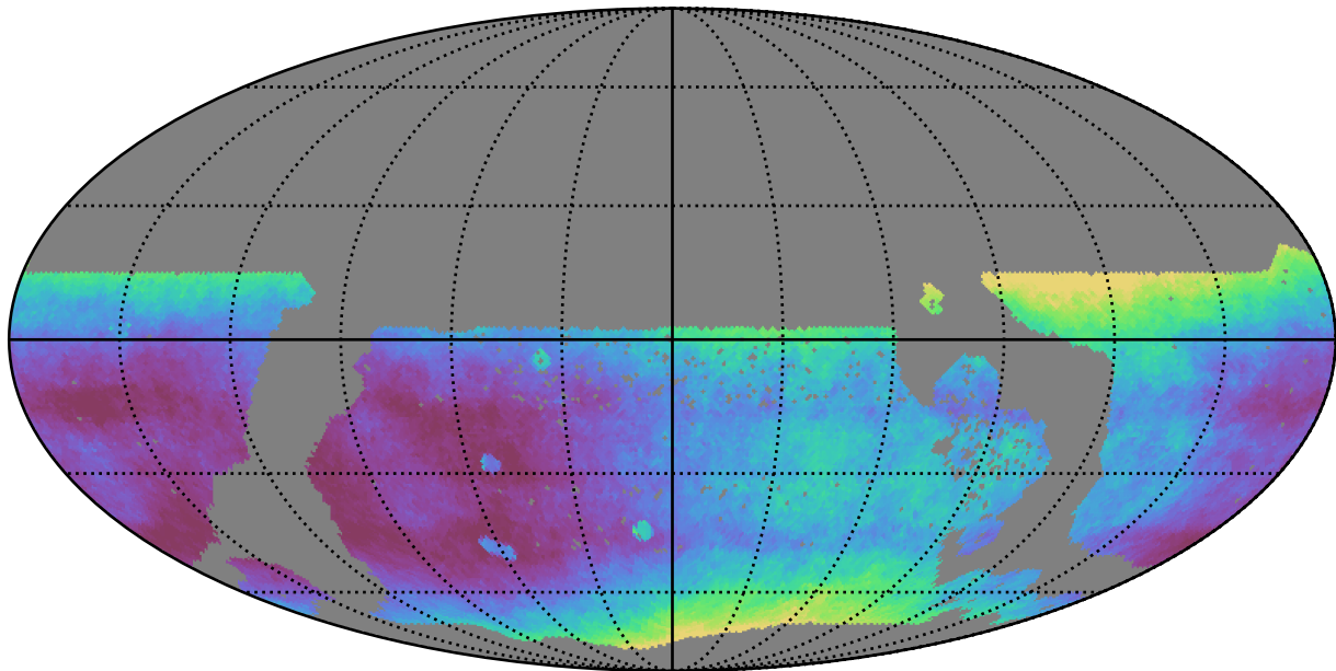
too_elab_r16_d3_gz_v3.4_10yrs WFD all bands: Median seeingEff
