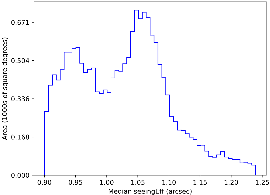
too_elab_r16_d3_gz_v3.4_10yrs WFD all bands: Median seeingEff
