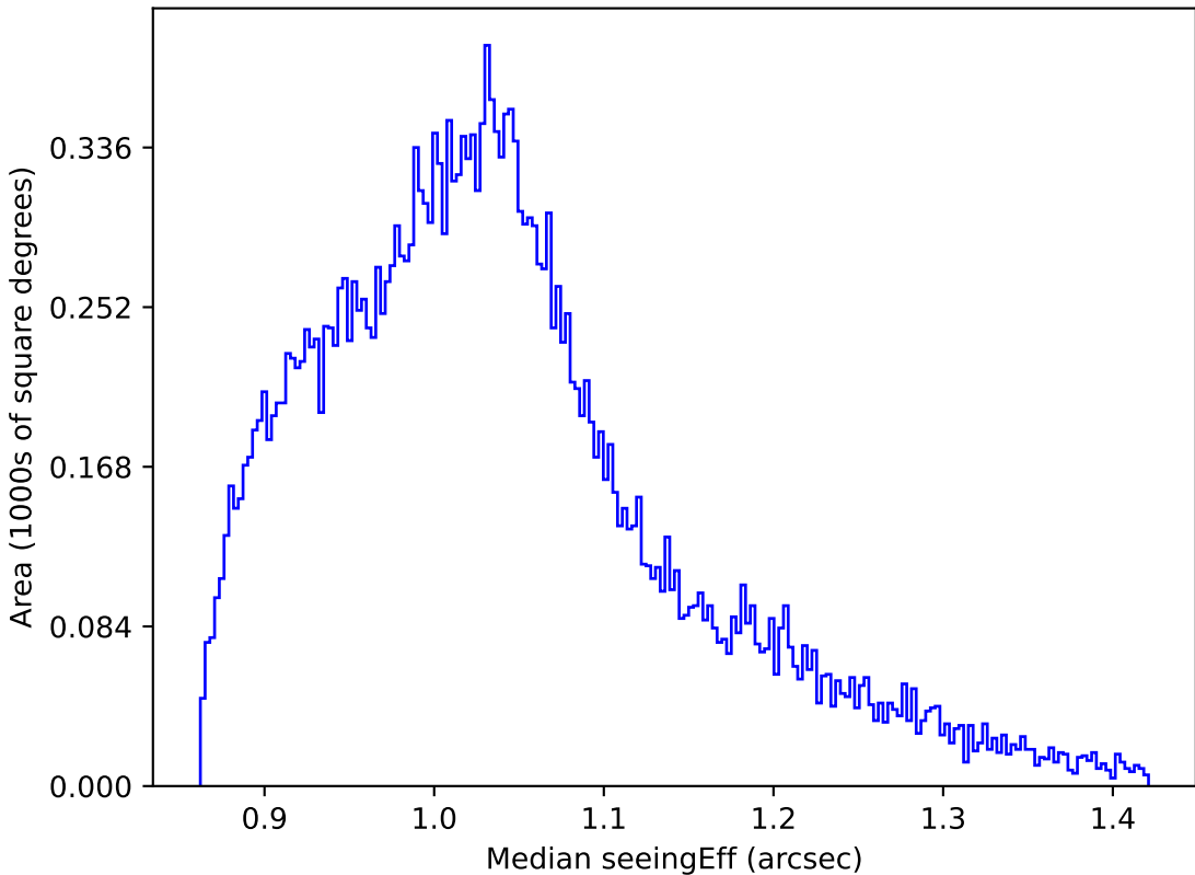
too_elab_r16_d3_gz_v3.4_10yrs All sky z band: Median seeingEff
